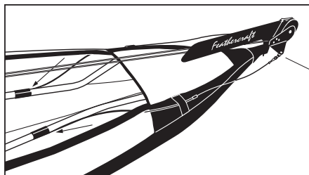
stern foot brace
